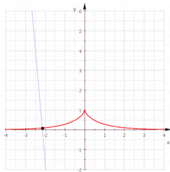
tractrix is a catenary
