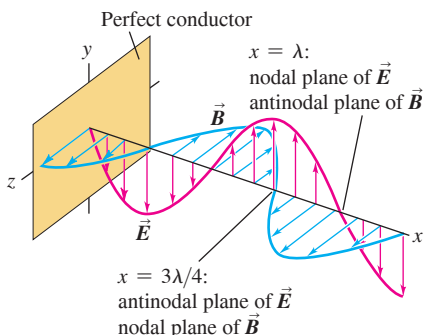
Figure 32.22 Representation of the electric and magnetic fields of a linearly polarized electromagnetic standing wave when \omega t = 3\pi/4 rad. In any plane perpendicular to the x -axis, E is maximum (an antinode) where B is zero (a node), and vice versa. As time elapses, the pattern does not move along the x -axis; instead, at every point the \vec{E} and \vec{B} vectors simply oscillate.
