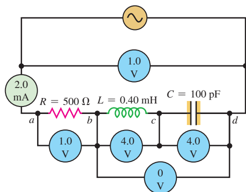
Figure 31.19 A radio tuning circuit at resonance. The circles denote rms current and voltages.
