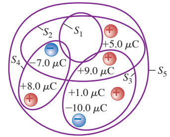
Figure 22.16 Five Gaussian surfaces and six point charges.
