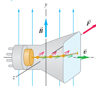
(b) If the tube axis is parallel to the x -axis, the beam is deflected in the -z -direction, so \vec{B} is in the +y -direction.
