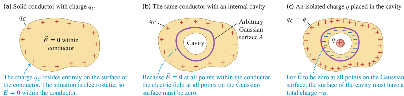
Figure 22.23 Finding the electric field within a charged conductor.
