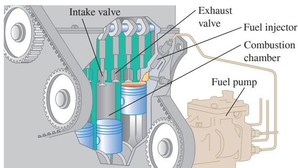
Figure 18.3 Cutaway of an automobile engine. While the air–petrol mixture is being compressed prior to ignition, both the intake and exhaust valves are in the closed (up) position.
