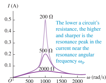
Figure 31.18 Graph of current amplitude I as a function of angular frequency \omega for an L - R - C series circuit with V = 100 V, L = 2.0 H, C = 0.50 \mu F, and three different values of the resistance R .
