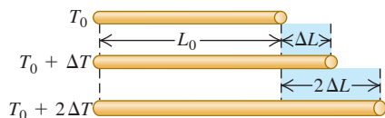
Figure 17.8 How the length of a rod changes with a change in temperature. (Length changes are exaggerated for clarity.)
