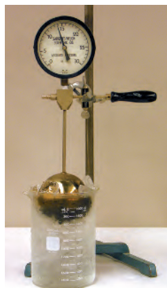
(a) A constant-volume gas thermometer
