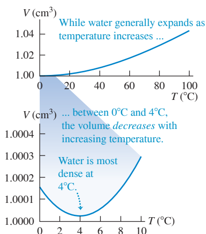
Figure 17.12 The volume of 1 gram of water in the temperature range from 0°C to 100°C. By 100°C the volume has increased to 1.043 cm 3 . If the coefficient of volume expansion were constant, the curve would be a straight line.
