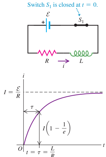
Figure 30.12 Graph of i versus t for growth of current in an R - L circuit with an emf in series. The final current is I = \mathcal{E}/R ; after one time constant \tau , the current is 1 - 1/e of this value.
