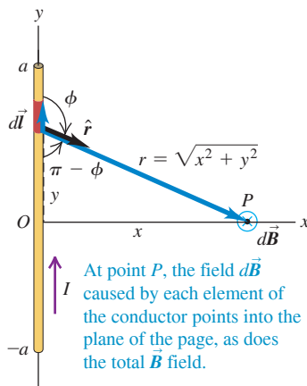
Figure 28.5 Magnetic field produced by a straight current-carrying conductor of length 2a .
