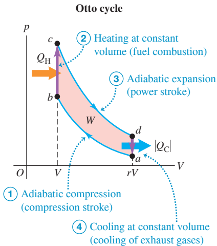
Figure 20.6 The pV -diagram for the Otto cycle, an idealized model of the thermodynamic processes in a petrol engine.
