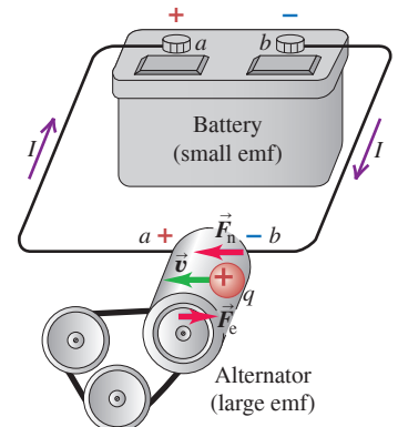
Figure 25.23 When two sources are connected in a simple loop circuit, the source with the larger emf delivers energy to the other source.
