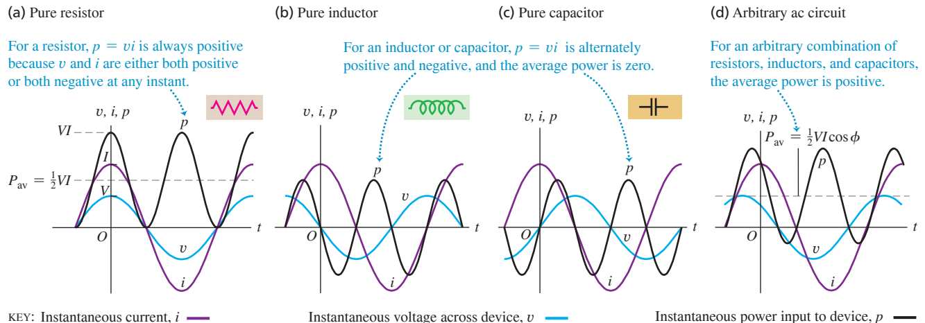
Figure 31.15 Graphs of current, voltage, and power as functions of time for (a) a pure resistor, (b) a pure inductor, (c) a pure capacitor, and (d) an arbitrary ac circuit that can have resistance, inductance, and capacitance.
