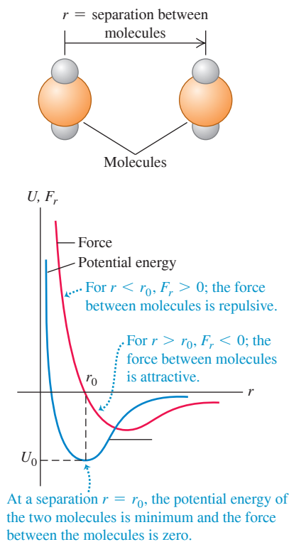
Figure 18.8 How the force between molecules and their potential energy of interaction depend on their separation r .
