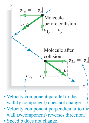
Figure 18.11 Elastic collision of a molecule with an idealized container wall.
