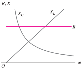
Figure 31.10 Graphs of R , X_L , and X_C as functions of angular frequency \omega .
