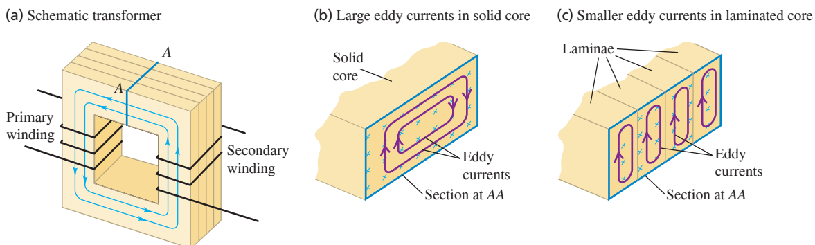
Figure 31.23 (a) Primary and secondary windings in a transformer. (b) Eddy currents in the iron core, shown in the cross section at AA. (c) Using a laminated core reduces the eddy currents.
